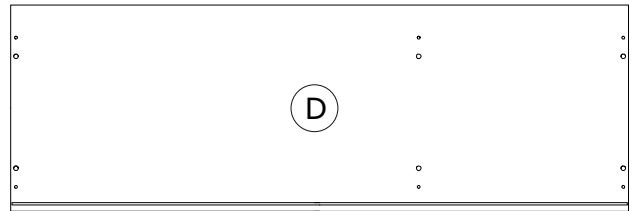
BA02540 1060x354x16mm
