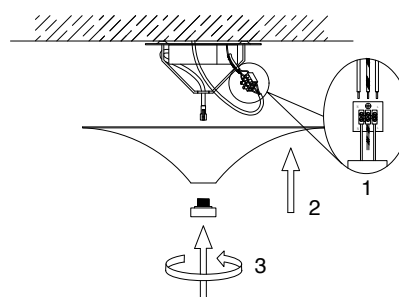
4. Connect the wires & rotate the metal cap
