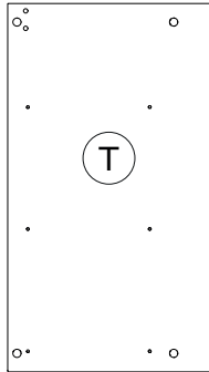
TR02686 676x372x16mm
