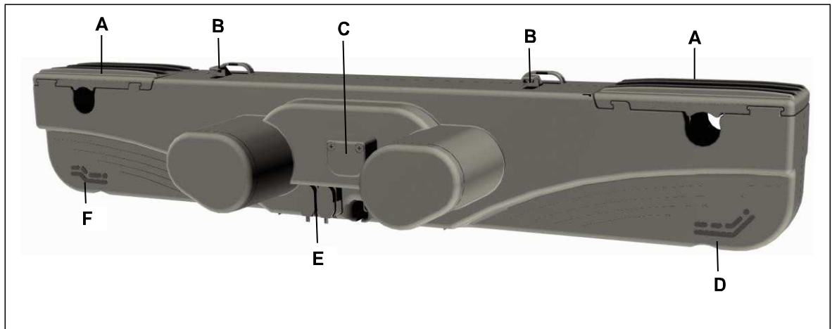
Figure 5 Main components of the OKIMAT 6 & OKIMAT 6B double drive (variant with detachable power cord)
