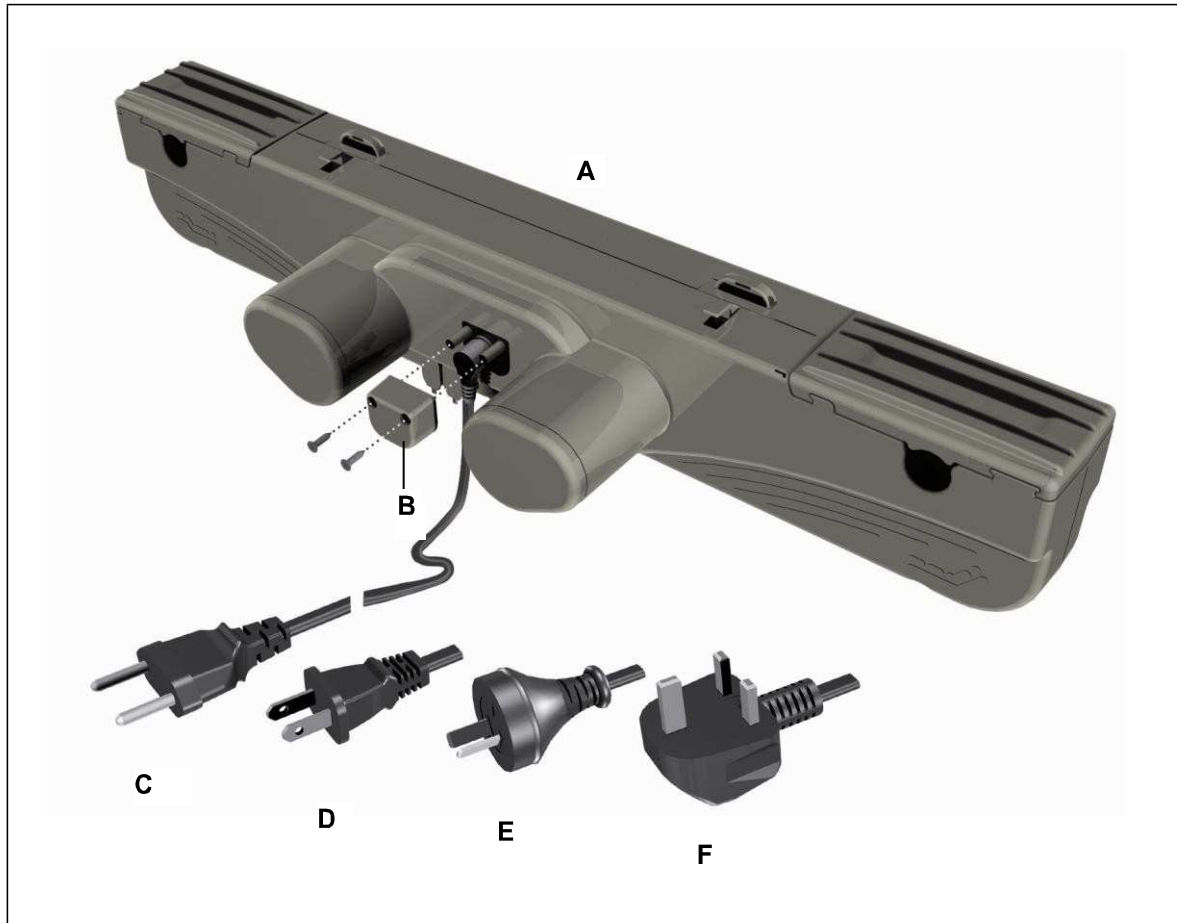
Figure 8 Power plug adapter, regional variants
