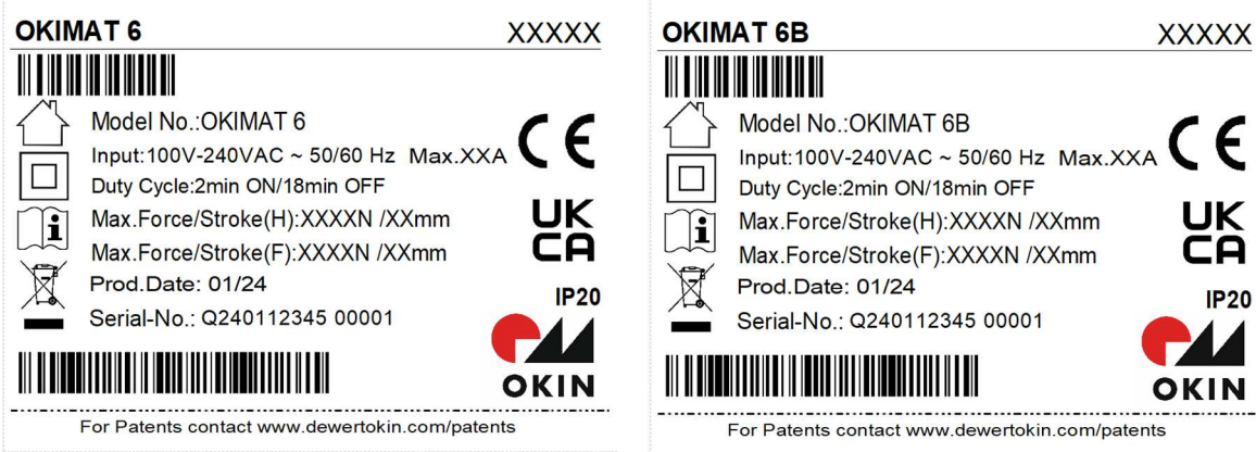
Figure 3 Ratings plate example
