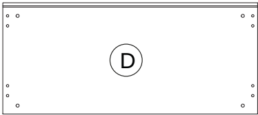
BA1946 816x357x30mm
