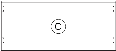
CA3203 816x357x30mm
