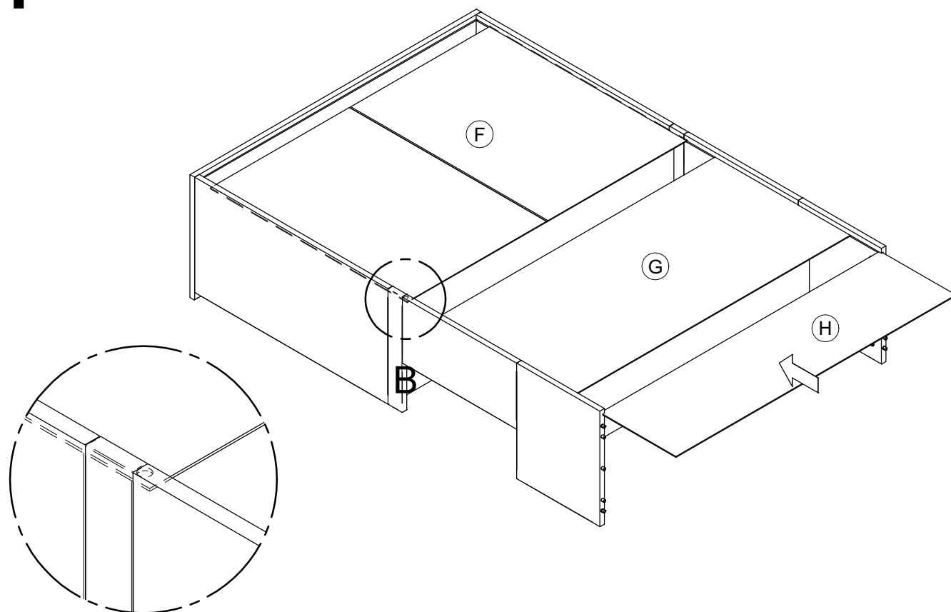
DETAIL B
