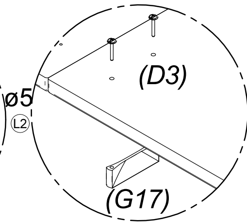
DETAIL E
