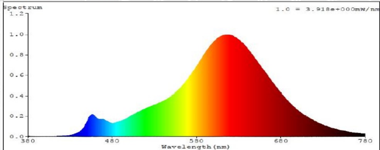
Model: 97260 (2200K)
