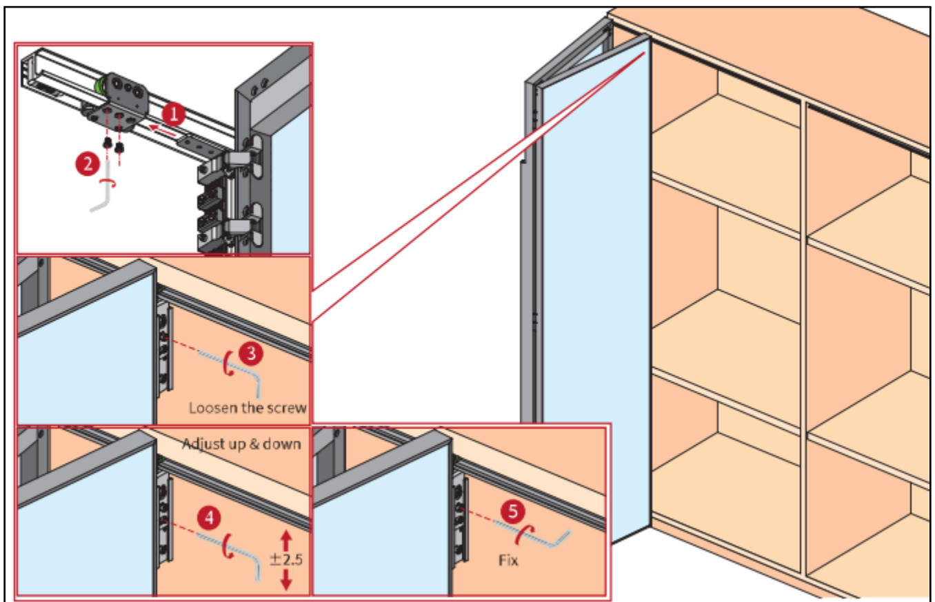
Justieren des Türblatts Adjust the balance of the door panel
