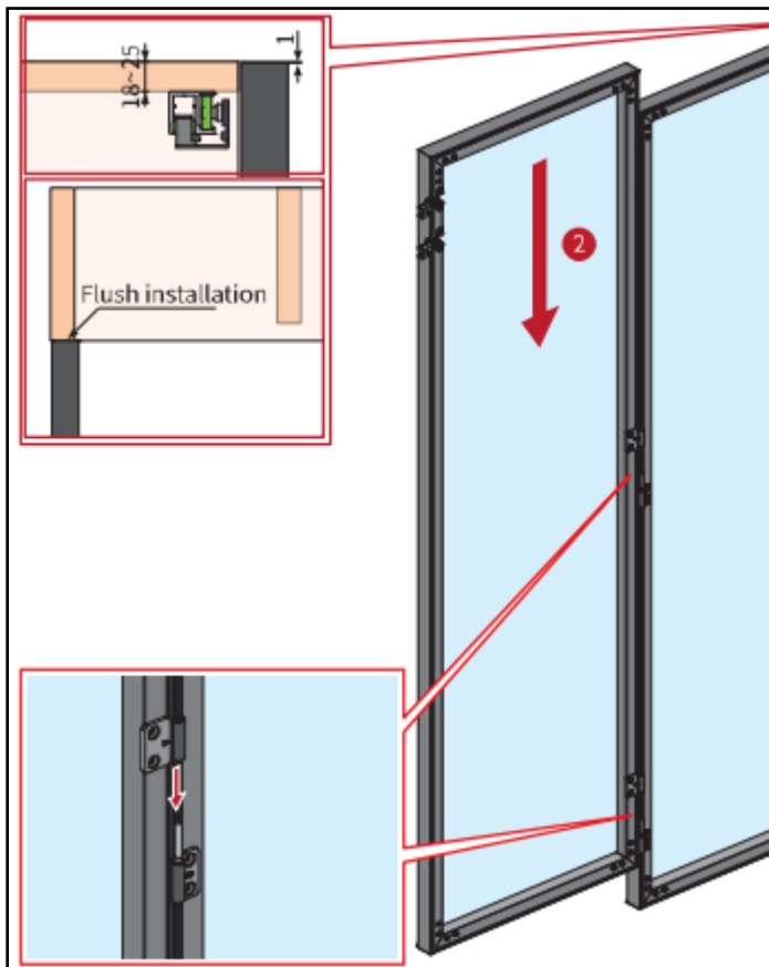
Tür einbauen Install door panel
