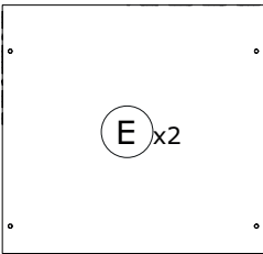
PI7958 335x318x16mm
