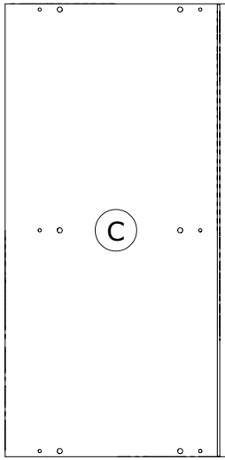
CA04201 720x353x16mm
