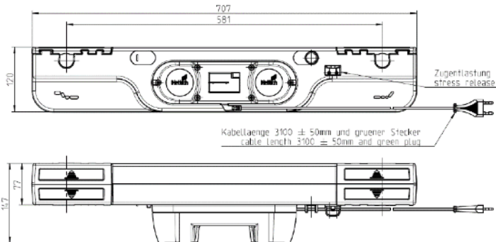
Abb. 8: AxisDrive IPS
