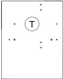
TR02633 478x372x16mm
