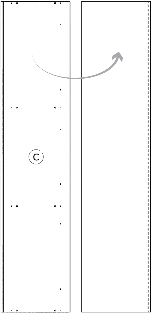
CA04138 1828x407x16mm
