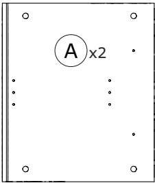
FI09859 478x405x16mm
