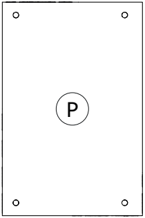
PI07867 564x371x16mm
