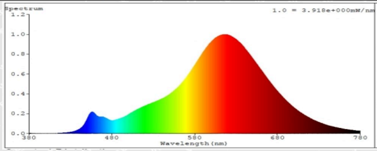
Model: 97200 (2200K)
