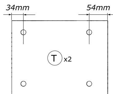
TR02682 218x280x16mm
