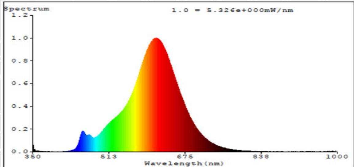
Model: 97310 (2200K)
