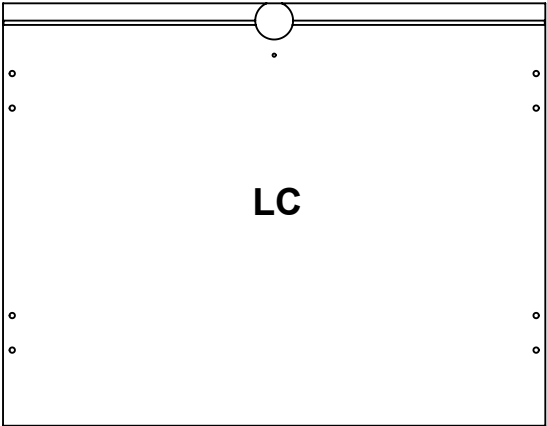
502x391x15mm
