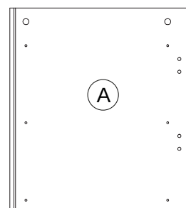
F17801 506x449x30mm
