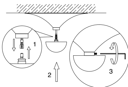
5. Connect the plug & fix in to place The cover with the metal cap
