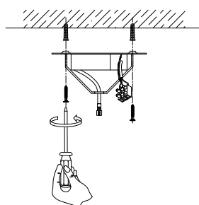
3. Drill holes & apply plastic anchors & screws
