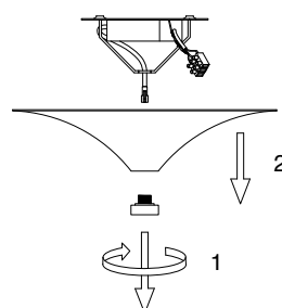
2. Rotate the metal cap to detach
