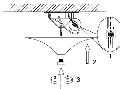
4. Connect the wires & rotate the metal cap
